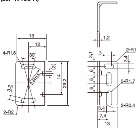
Standard Bracket for cable type (BEF-W150-A)
