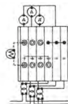
THREE PHASE CT TEST
