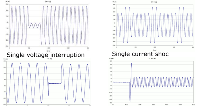
CP11B output signals recorded by digital oscilloscope
